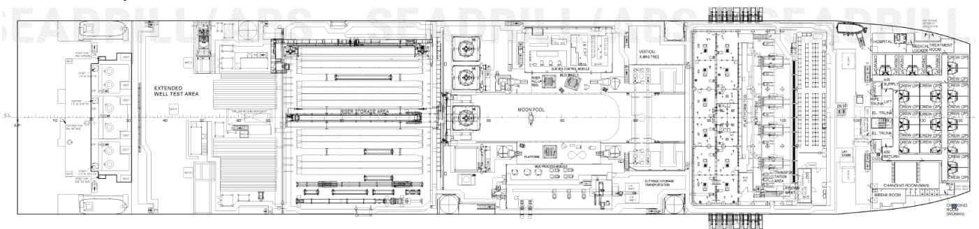
West Carina – Top View
