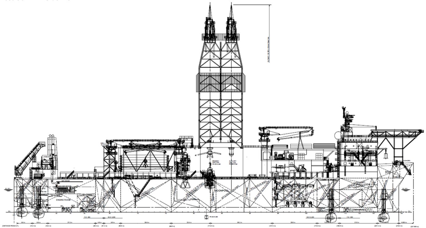
West Gemini – Side View
